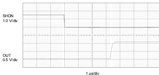
Figure 7. Startup Delay
