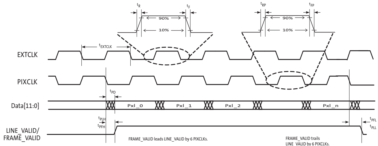
Figure 12: I/O Timing Diagram
