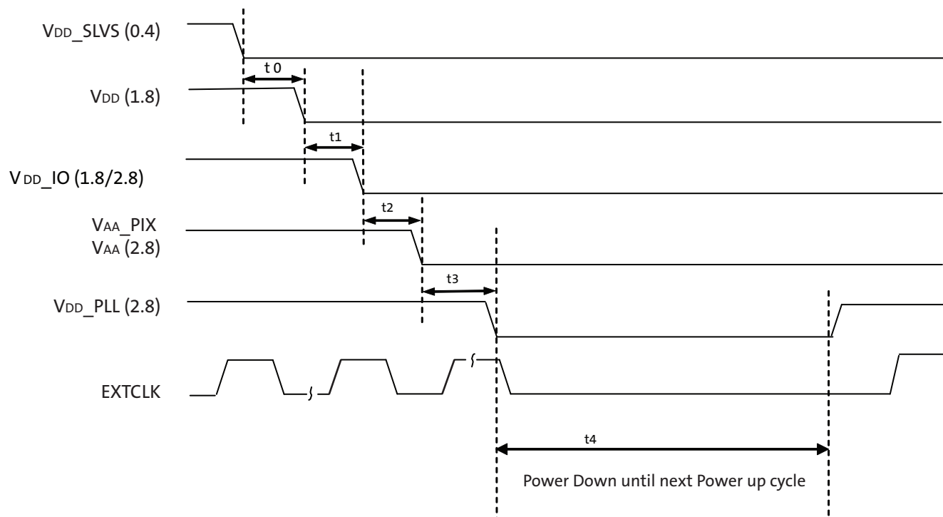
Figure 14: Power Down
