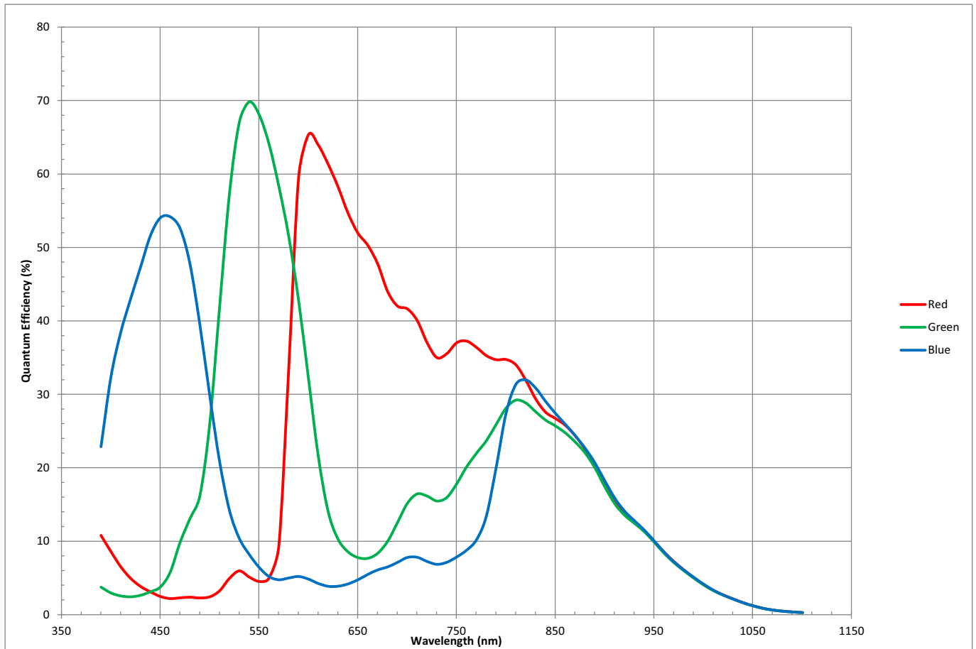
Figure 10: Quantum Efficiency
