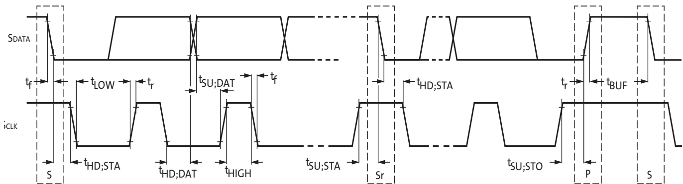
Figure 11: Two-Wire Serial Bus Timing Parameters
