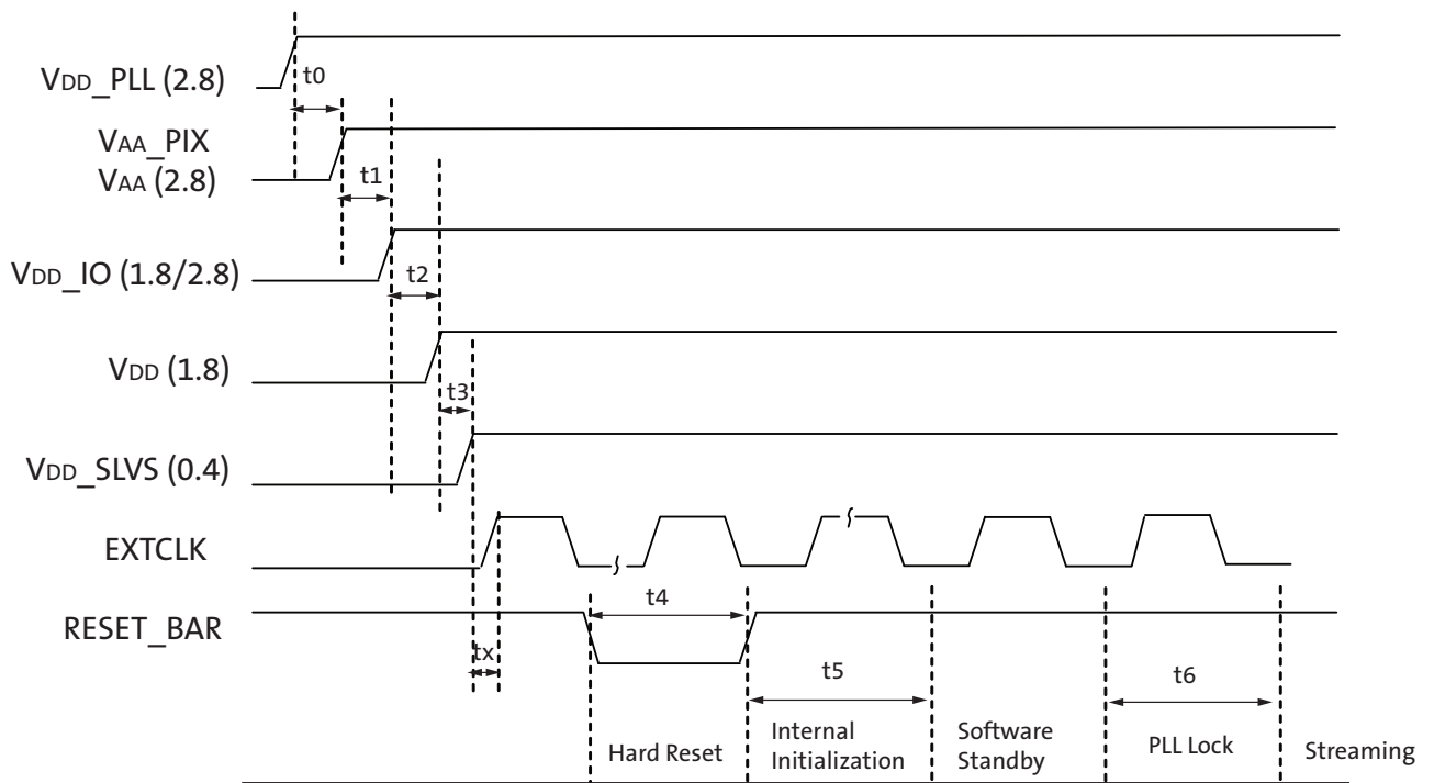
Figure 13: Power Up
